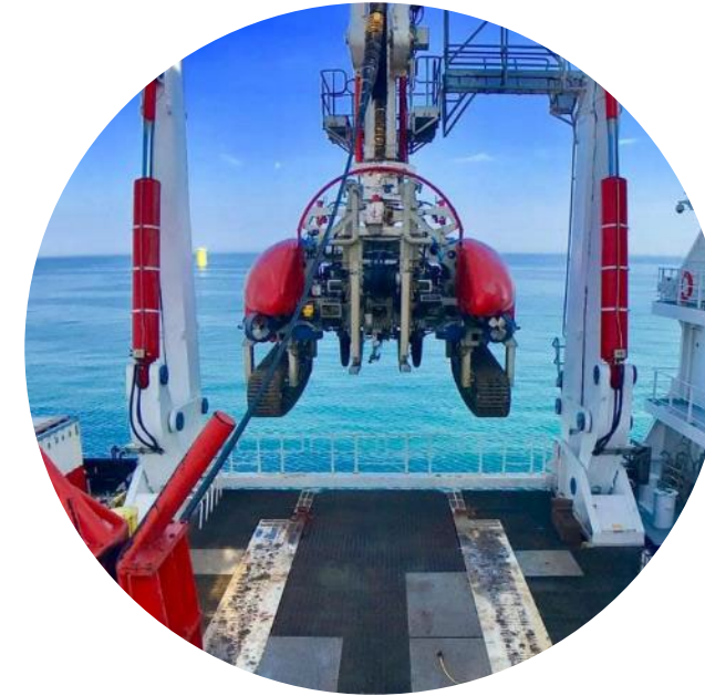
Subsea Trenchers (6 units) Four jet trenchers, one cutting trencher and one plough trencher
