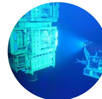
Intervention Riser Systems Utilized for wireline intervention, production logging, coiled-tubing operations, well stimulation and full P&A operations
